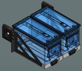
Ammo box holder M19A1 (Cal 7,62mm) M2A1 (Cal 12,7mm) PA120 (Cal 40mm)
