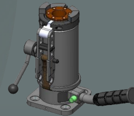
Pintle Interface - Jacking
