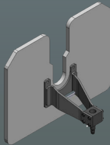
Ballistic Shield HMG Level 2/3
